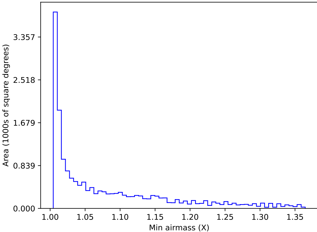
smc_Imc_v3.3_10yrs WFD all bands: Min airmass
