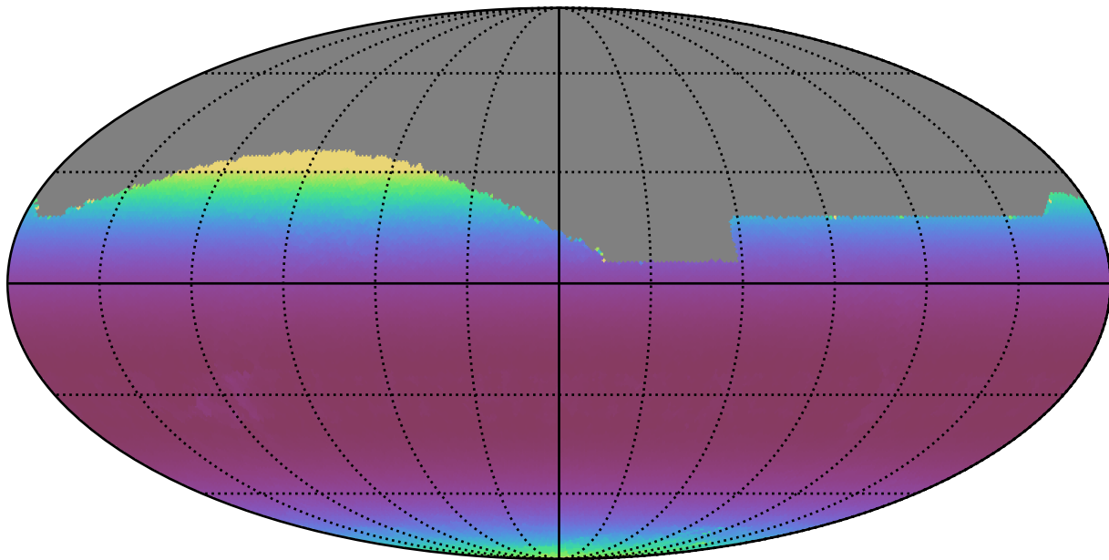
smc_lmc_v3.3_10yrs All sky z band: Min airmass
