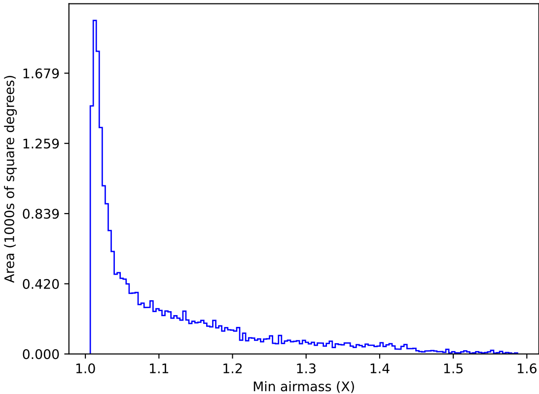
smc_lmc_v3.3_10yrs All sky y band: Min airmass
