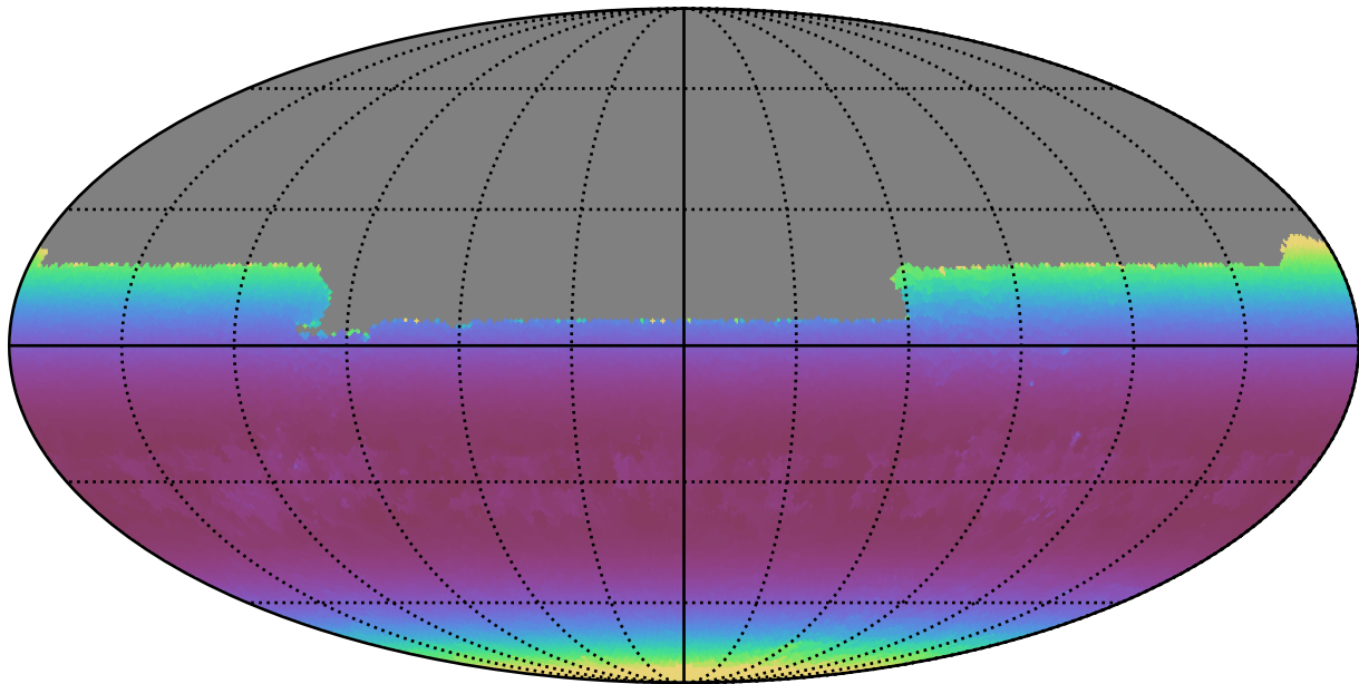
smc_lmc_v3.3_10yrs All sky u band: Min airmass
