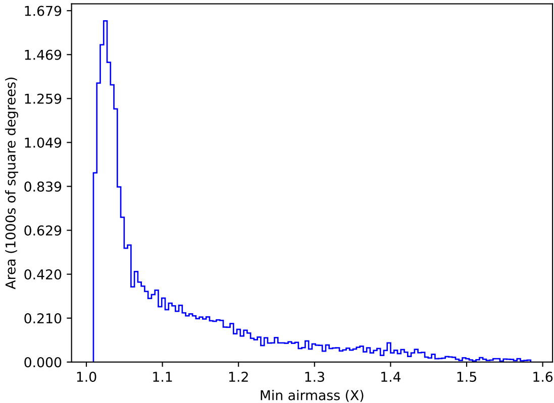
smc_lmc_v3.3_10yrs All sky u band: Min airmass
