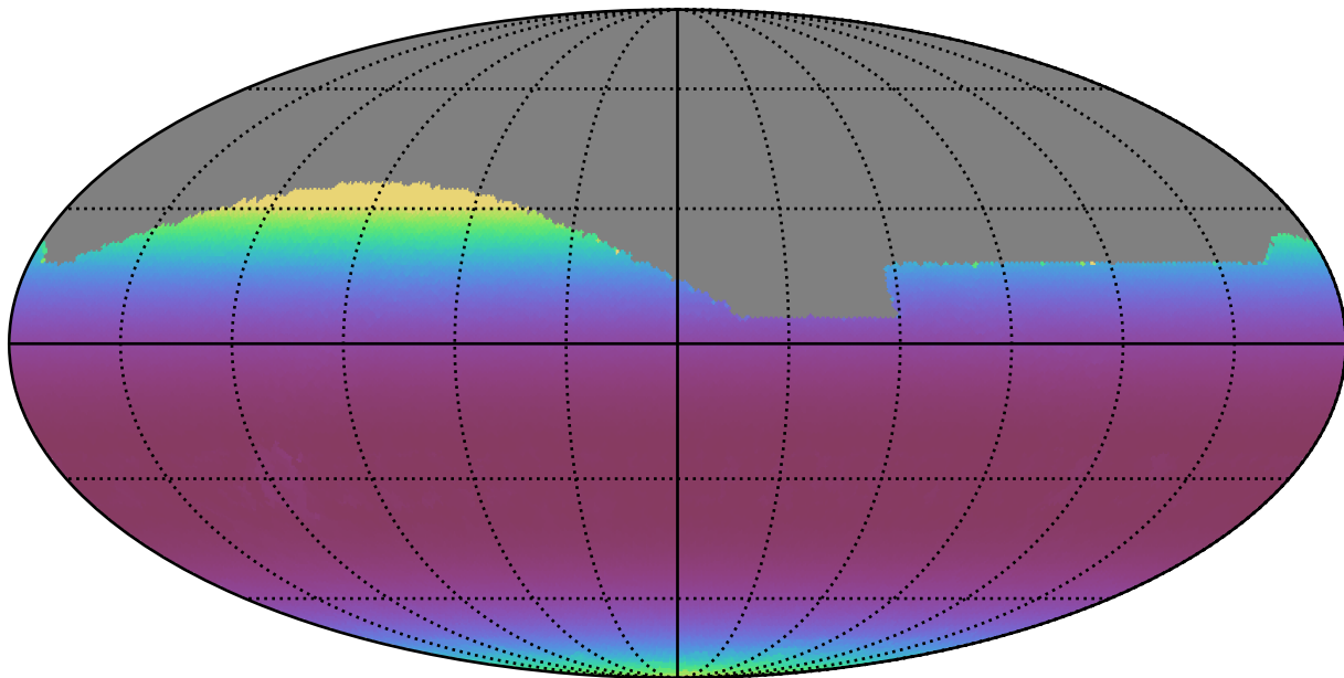
smc_lmc_v3.3_10yrs All sky r band: Min airmass
