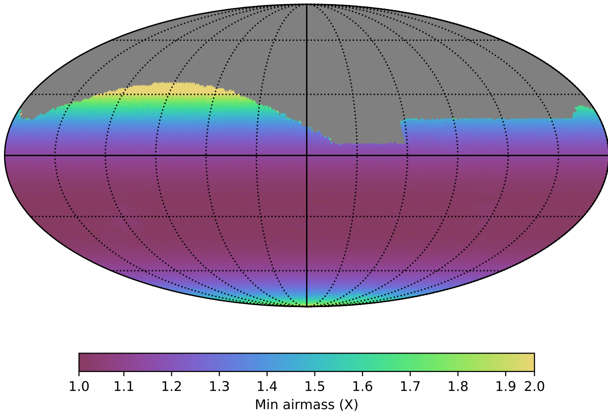
smc_lmc_v3.3_10yrs All sky i band: Min airmass
