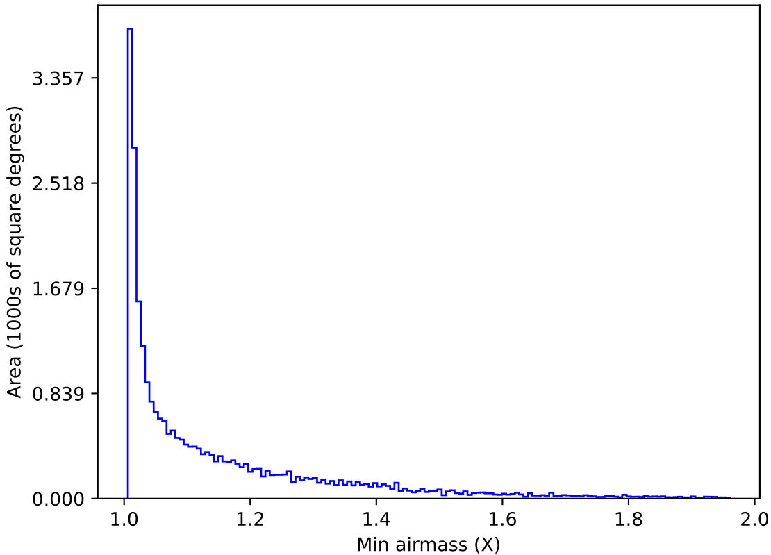
smc_lmc_v3.3_10yrs All sky i band: Min airmass
