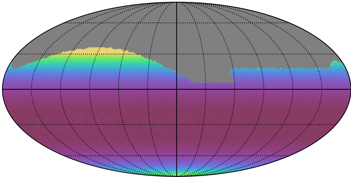
smc_lmc_v3.3_10yrs All sky g band: Min airmass
