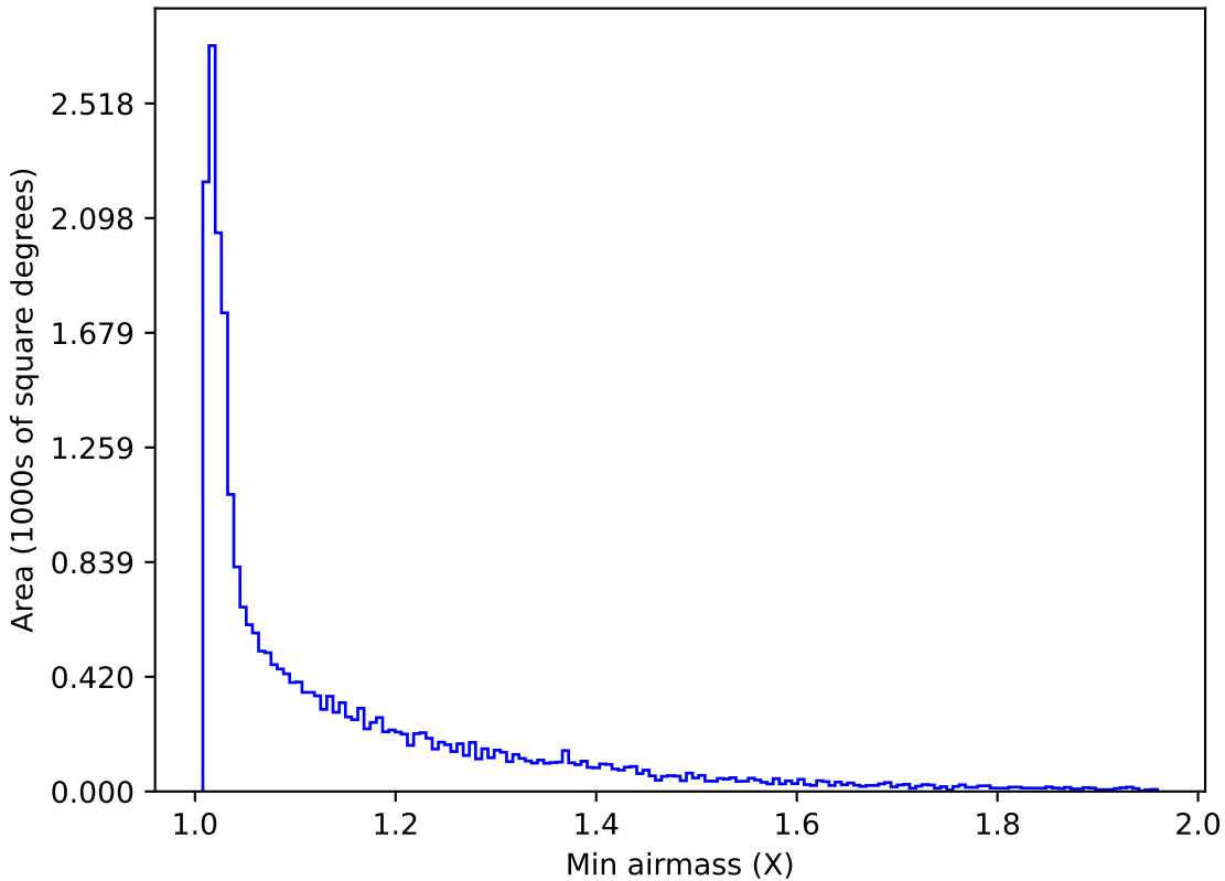
smc_lmc_v3.3_10yrs All sky g band: Min airmass
