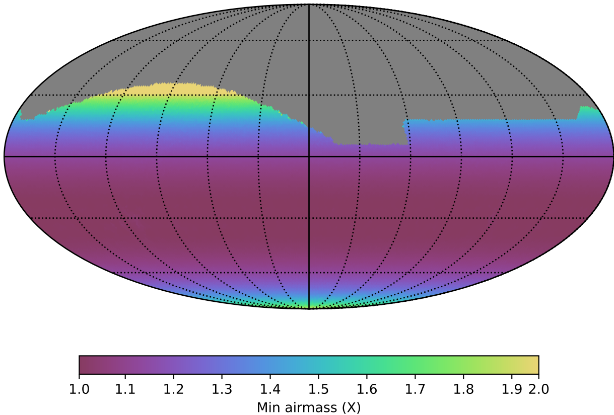
smc_lmc_v3.3_10yrs All sky all bands: Min airmass
