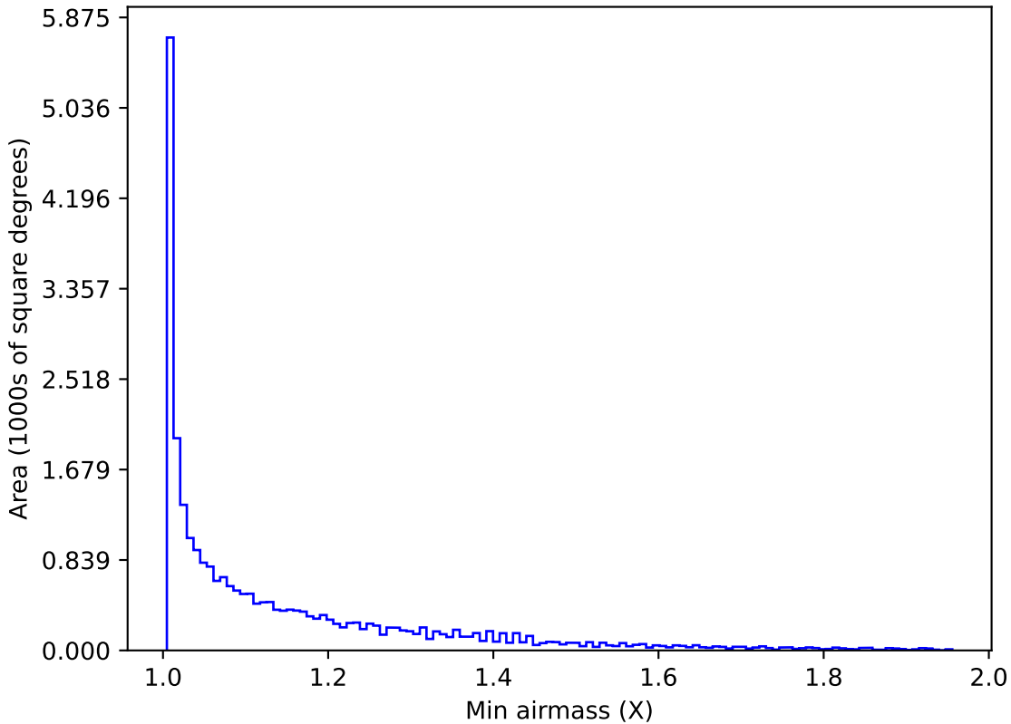
smc_lmc_v3.3_10yrs All sky all bands: Min airmass
