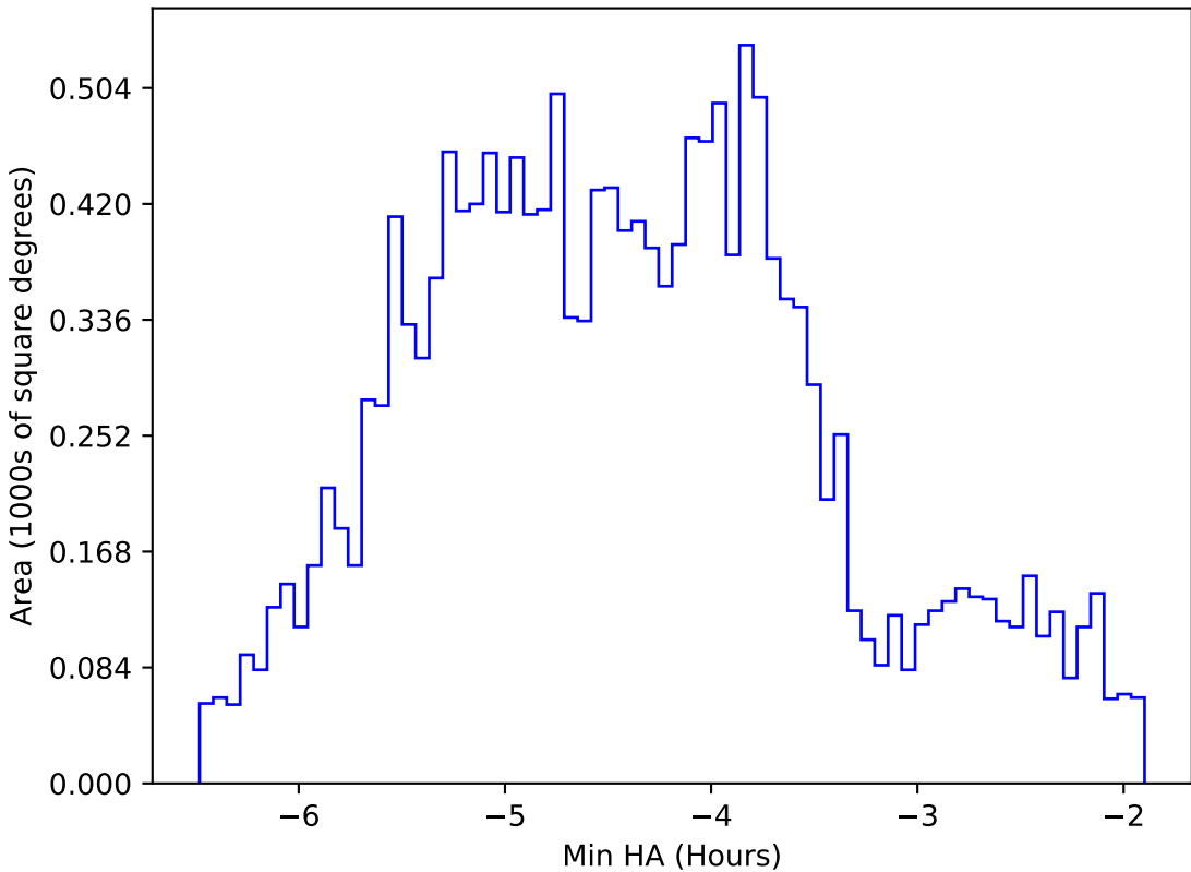
smc_lmc_v3.3_10yrs WFD z band: Min HA
