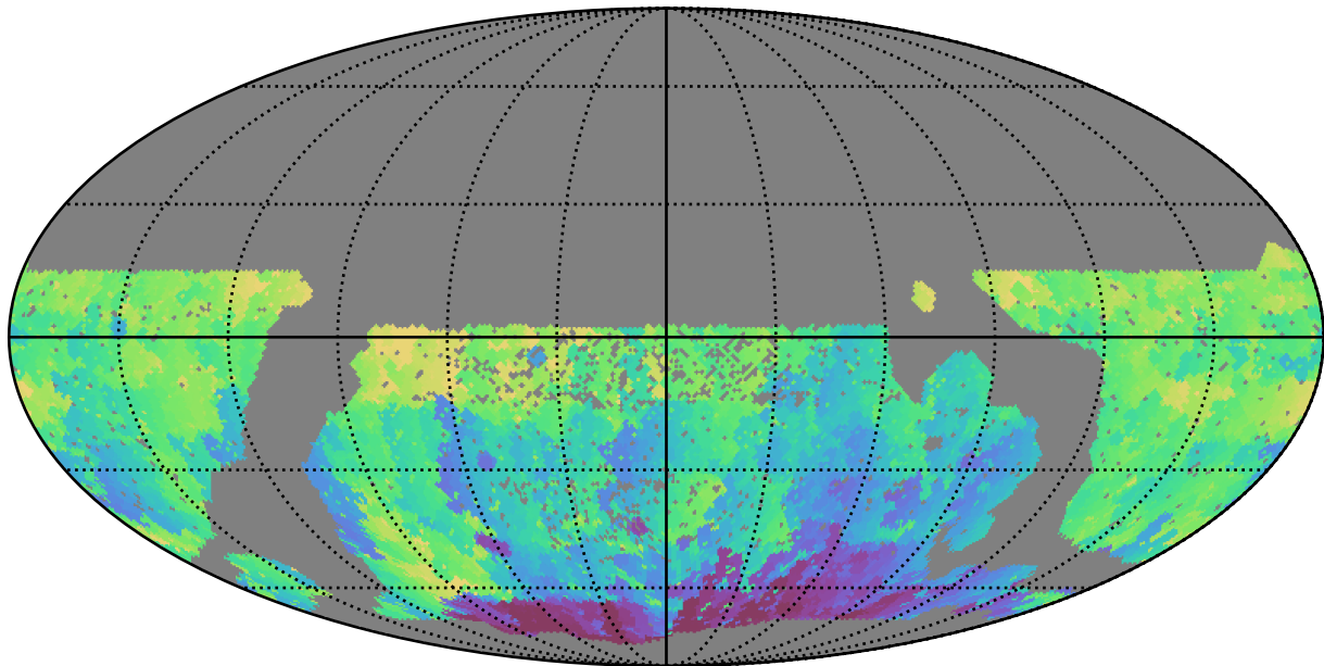
smc_lmc_v3.3_10yrs WFD u band: Min HA
