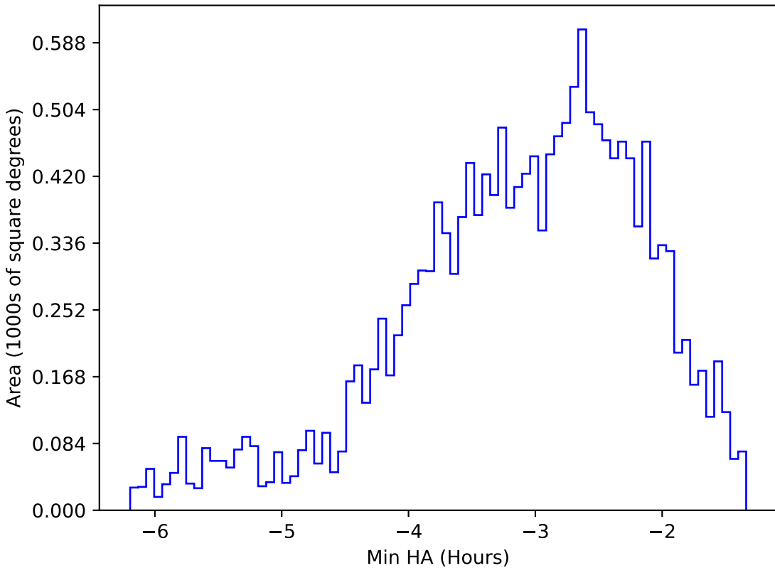
smc_lmc_v3.3_10yrs WFD u band: Min HA
