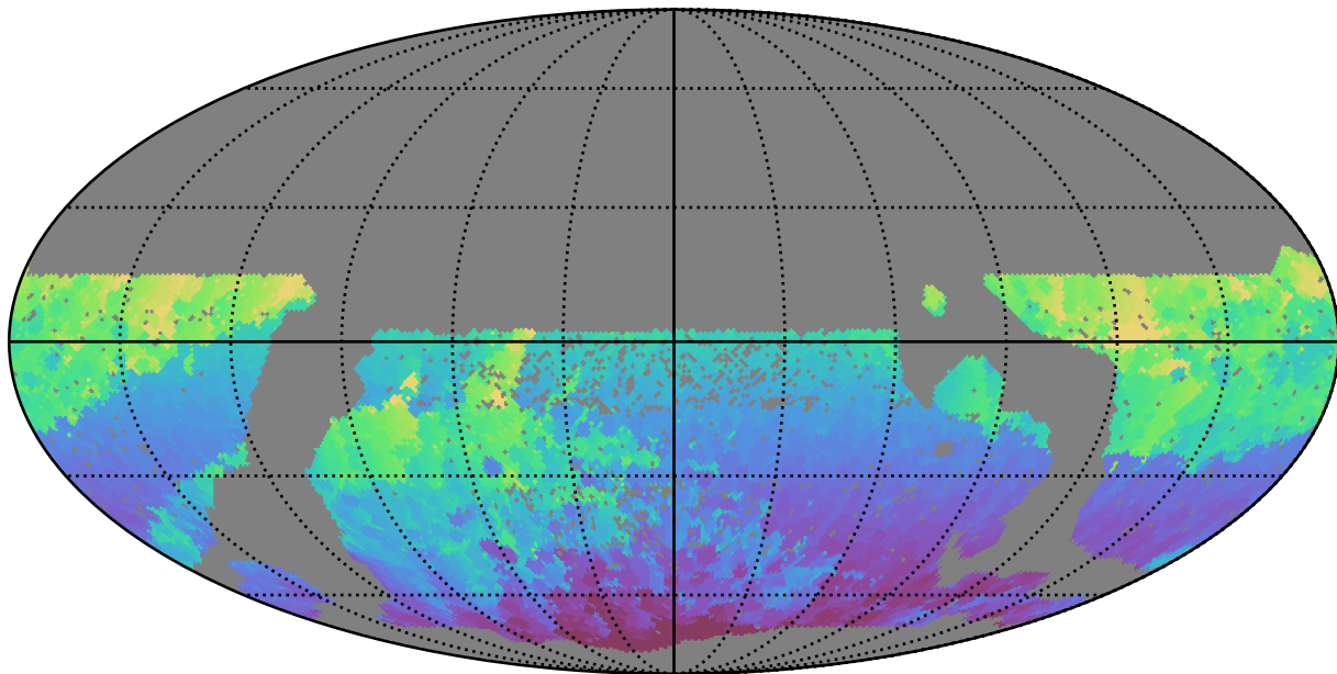
smc_lmc_v3.3_10yrs WFD r band: Min HA
