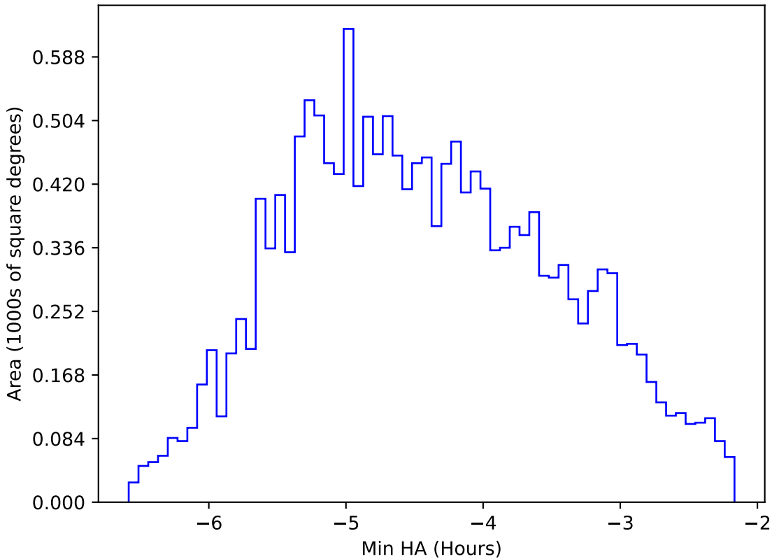
smc_lmc_v3.3_10yrs WFD r band: Min HA
