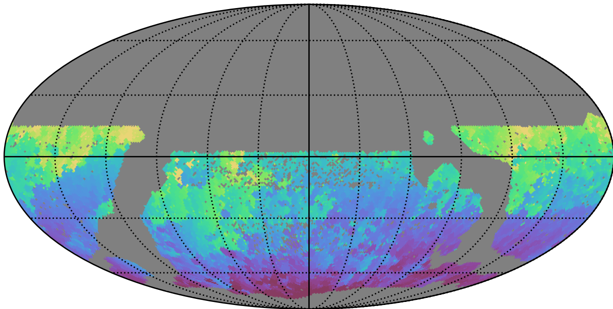
smc_lmc_v3.3_10yrs WFD i band: Min HA
