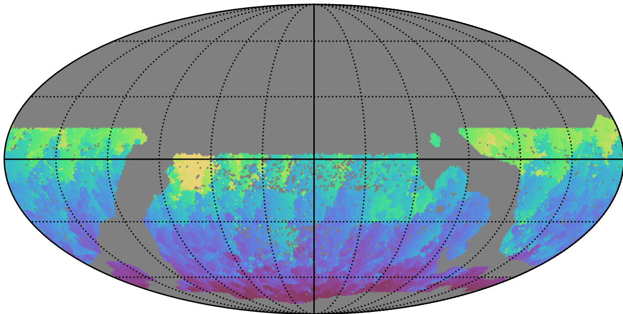
smc_lmc_v3.3_10yrs WFD g band: Min HA
