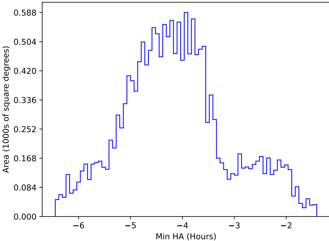
smc_lmc_v3.3_10yrs WFD g band: Min HA
