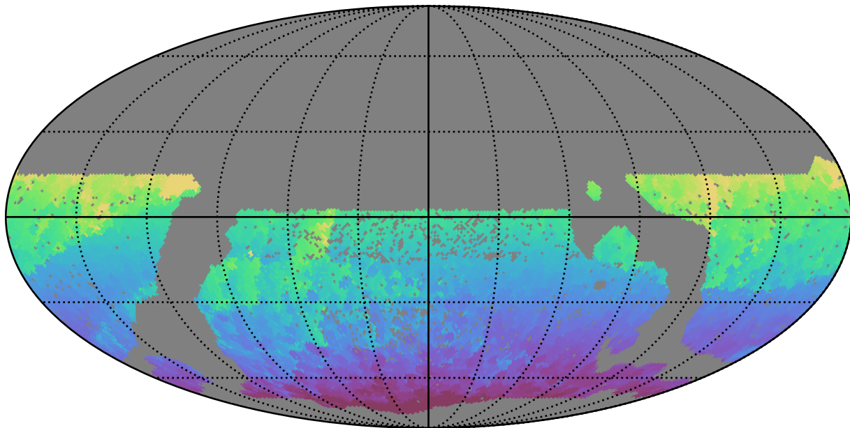
smc_lmc_v3.3_10yrs WFD all bands: Min HA
