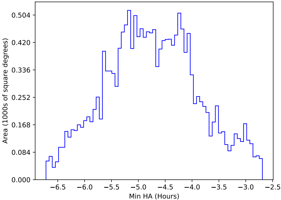
smc_lmc_v3.3_10yrs WFD all bands: Min HA
