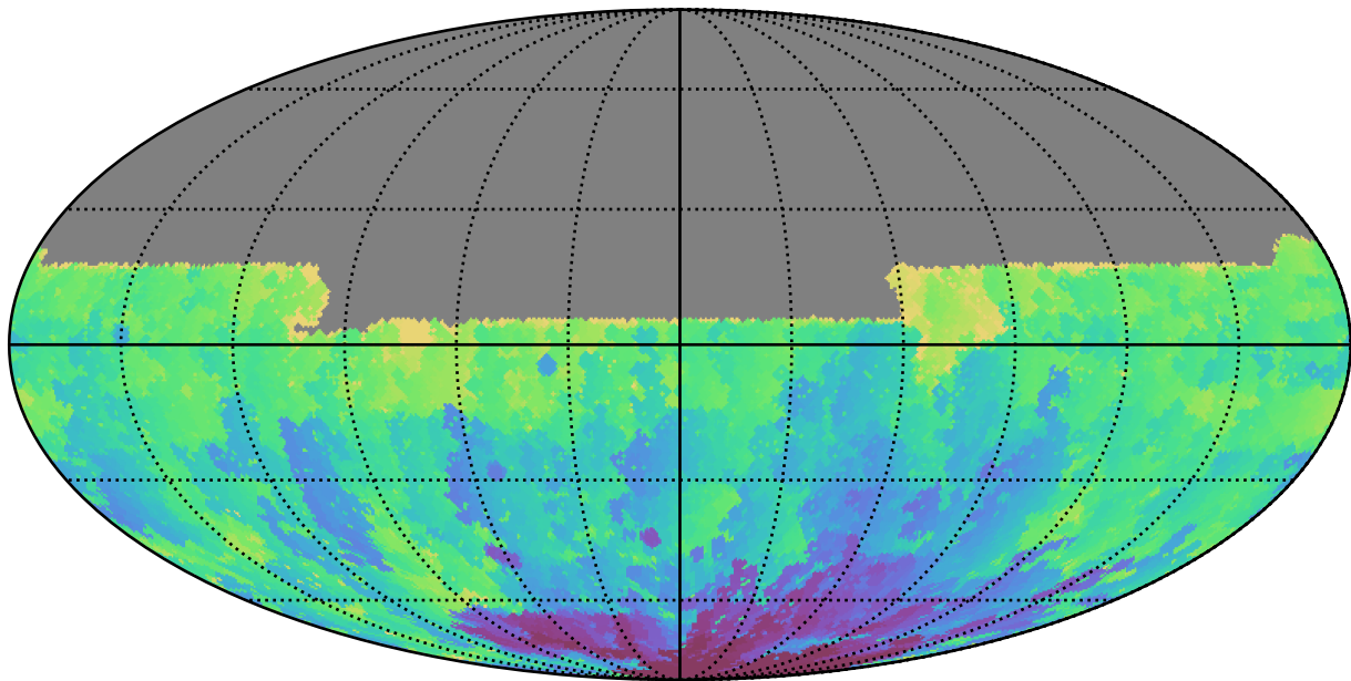
smc_lmc_v3.3_10yrs All sky u band: Min HA
