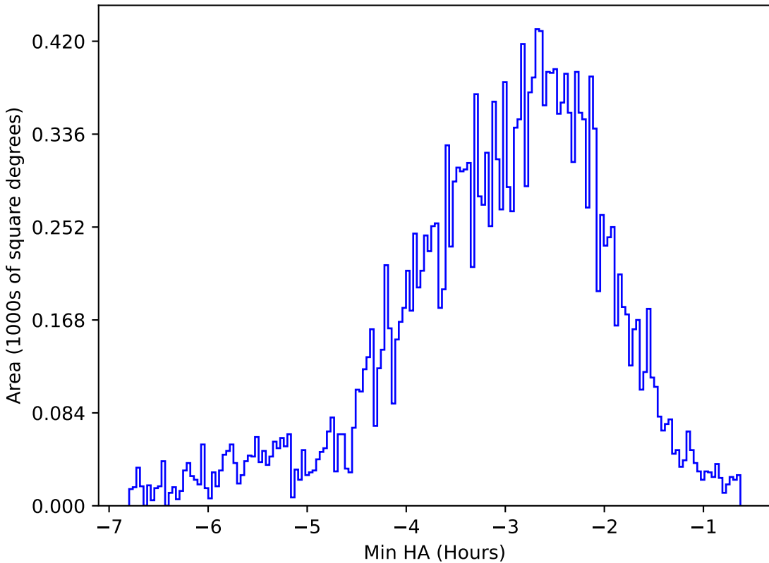
smc_lmc_v3.3_10yrs All sky u band: Min HA
