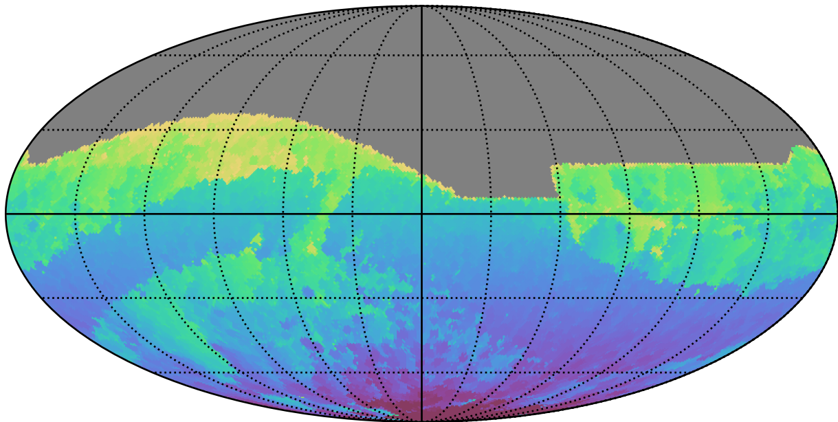
smc_lmc_v3.3_10yrs All sky r band: Min HA
