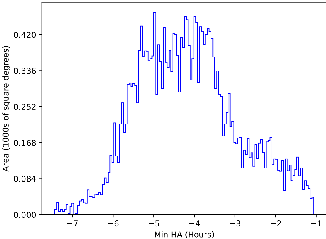
smc_lmc_v3.3_10yrs All sky r band: Min HA
