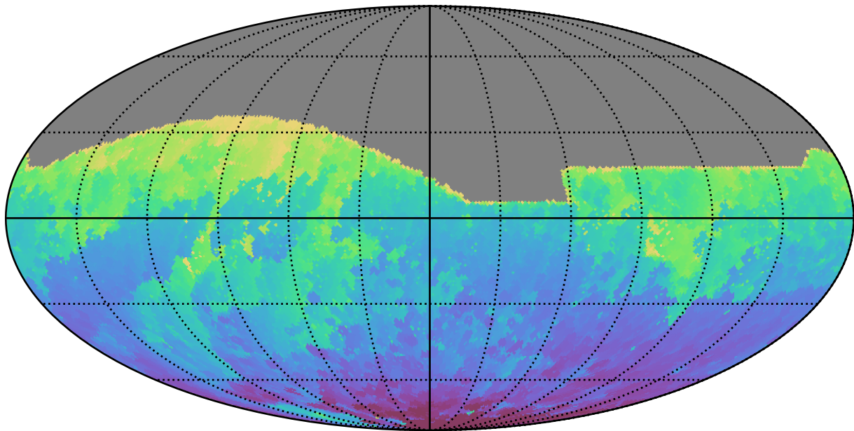
smc_lmc_v3.3_10yrs All sky i band: Min HA
