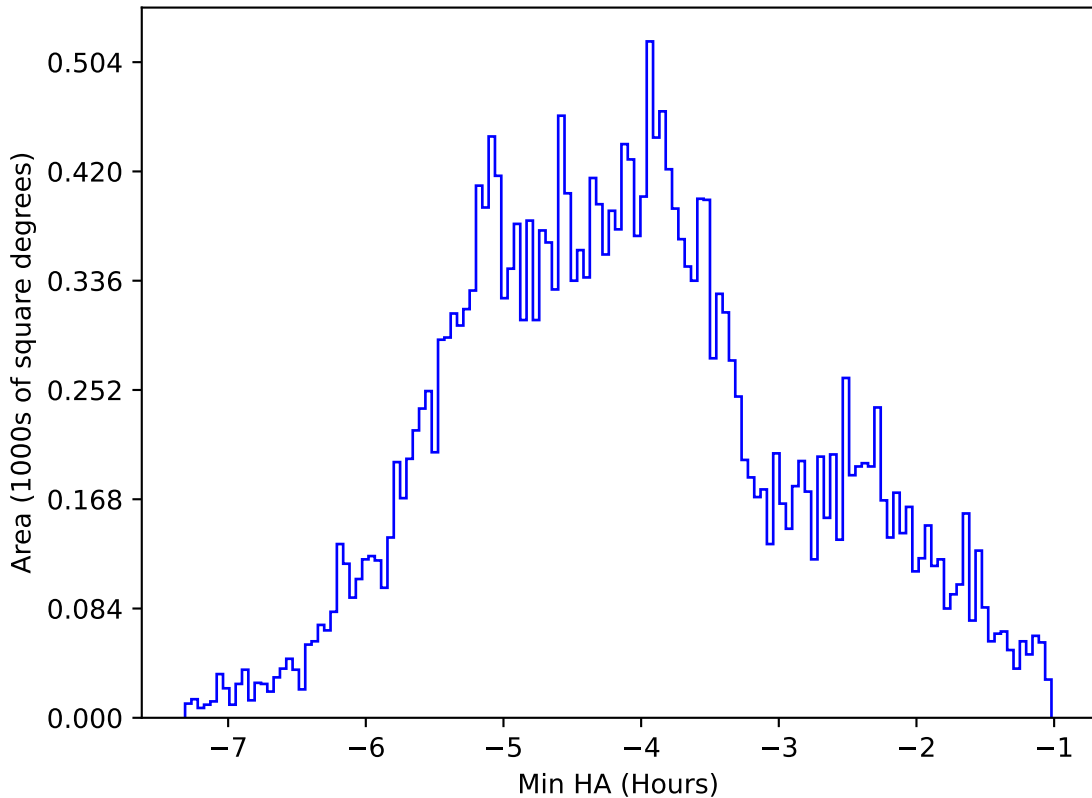
smc_lmc_v3.3_10yrs All sky i band: Min HA
