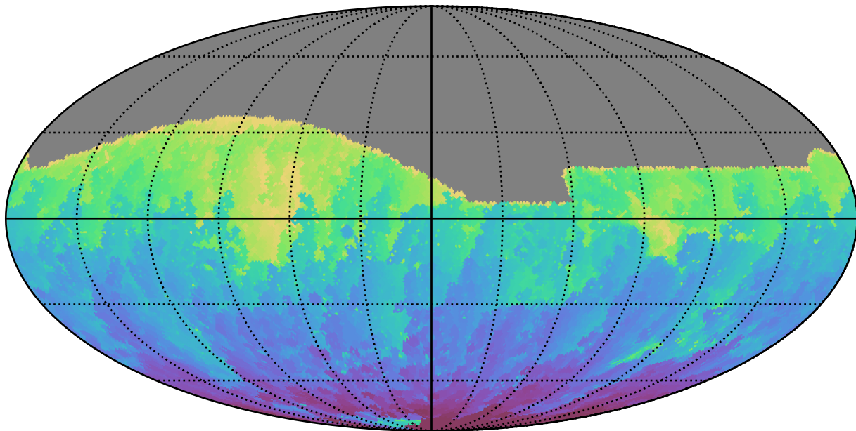
smc_lmc_v3.3_10yrs All sky g band: Min HA
