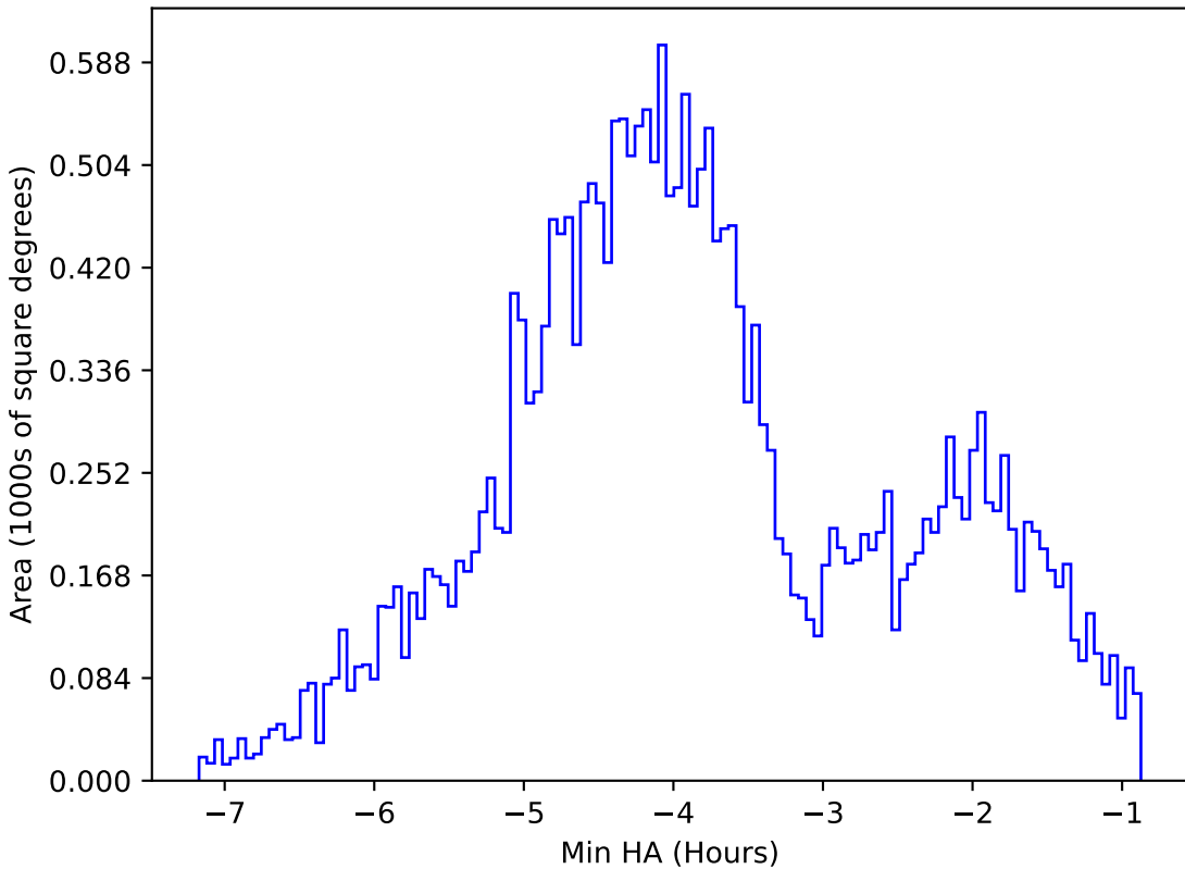
smc_lmc_v3.3_10yrs All sky g band: Min HA
