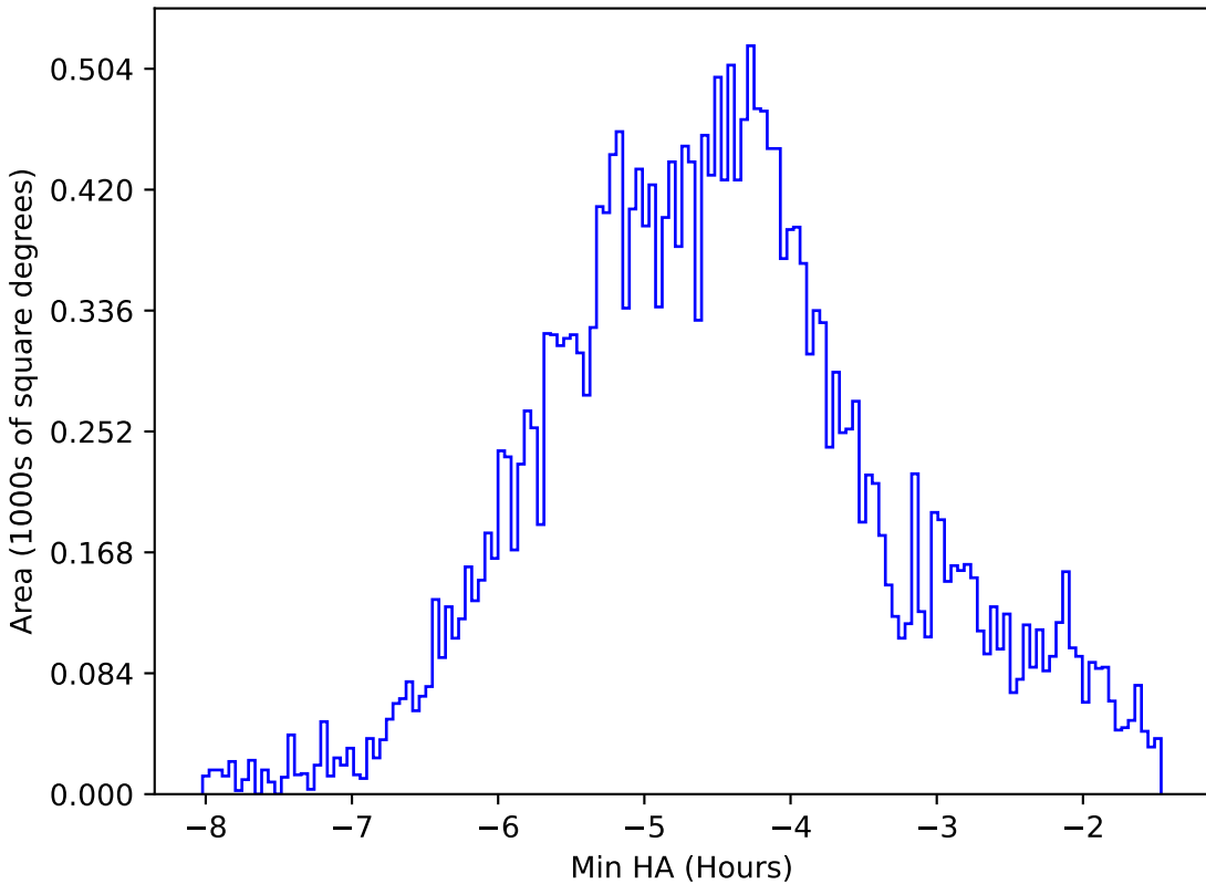
smc_lmc_v3.3_10yrs All sky all bands: Min HA
