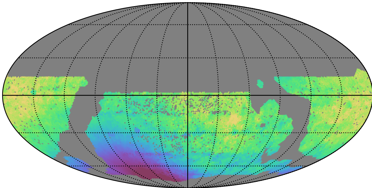
smc_lmc_v3.3_10yrs WFD z band: Median solarElong
