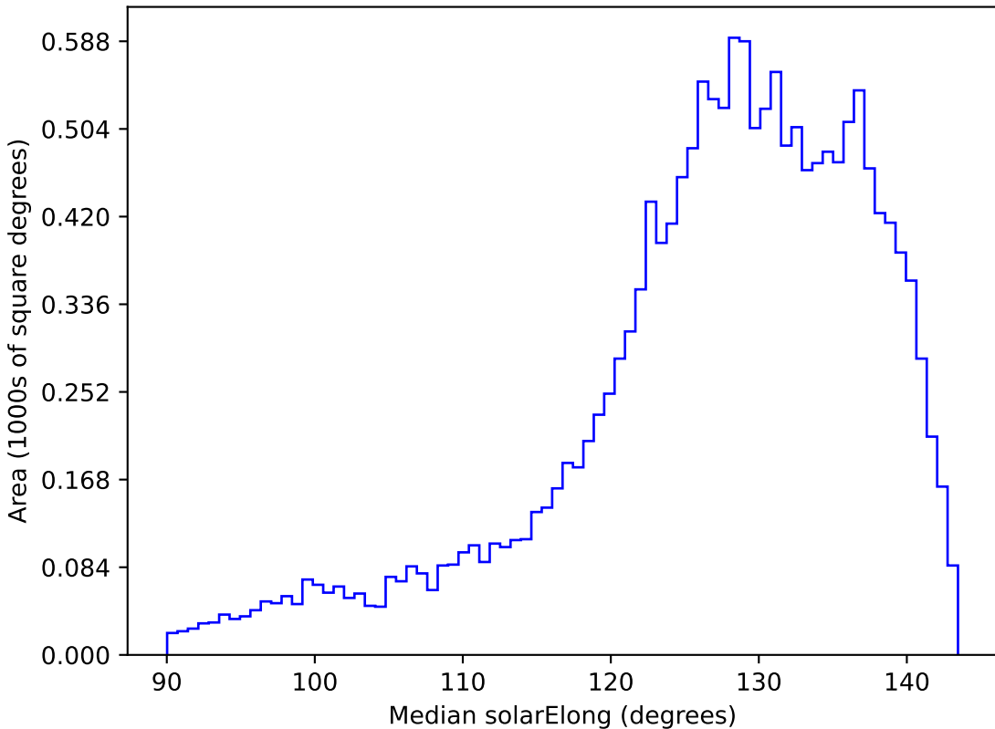
smc_lmc_v3.3_10yrs WFD z band: Median solarElong
