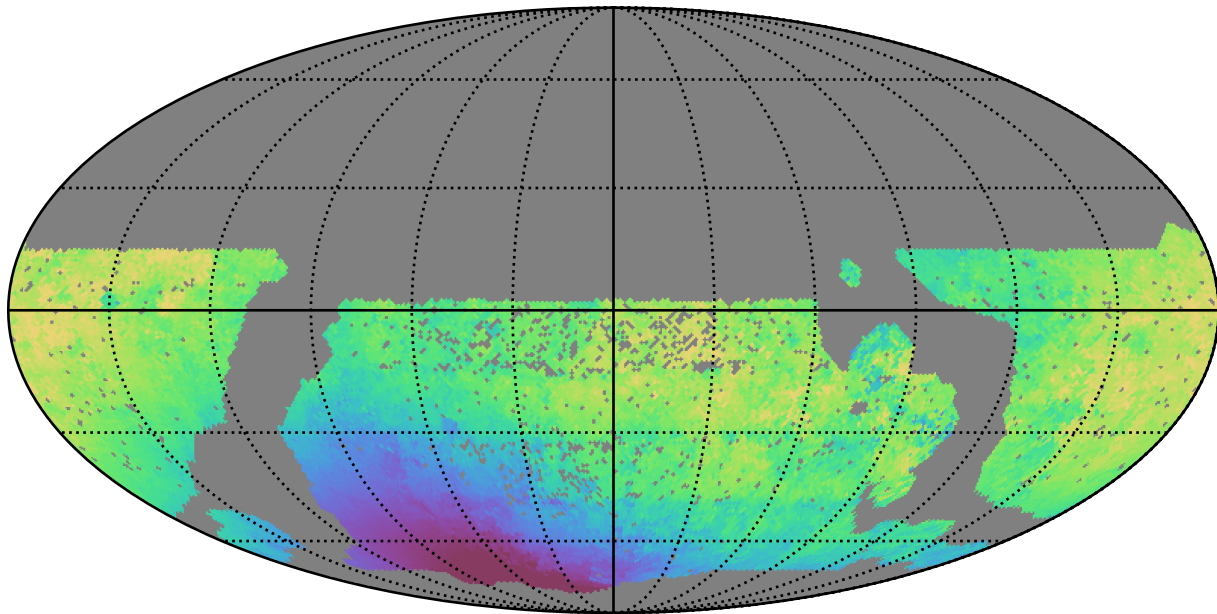
smc_lmc_v3.3_10yrs WFD y band: Median solarElong
