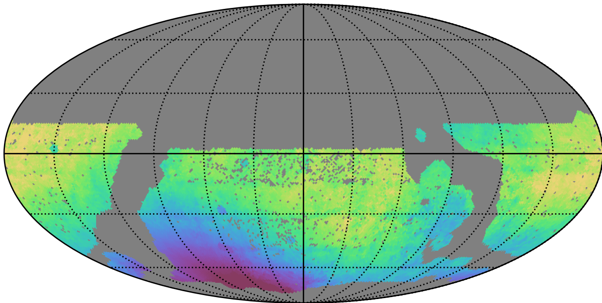
smc_lmc_v3.3_10yrs WFD r band: Median solarElong
