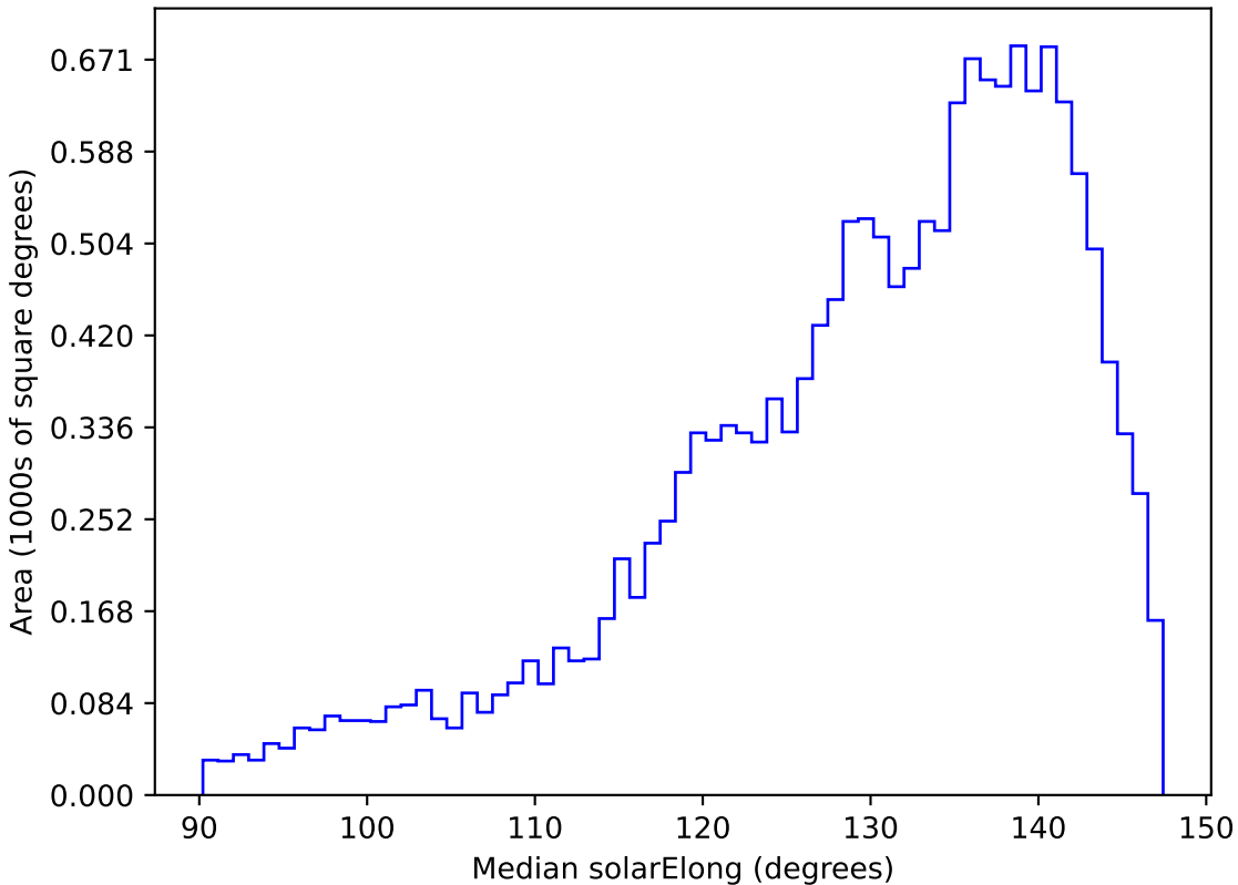
smc_lmc_v3.3_10yrs WFD r band: Median solarElong
