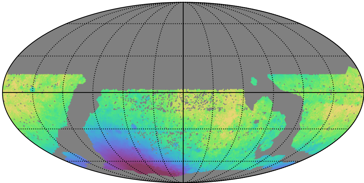
smc_lmc_v3.3_10yrs WFD i band: Median solarElong
