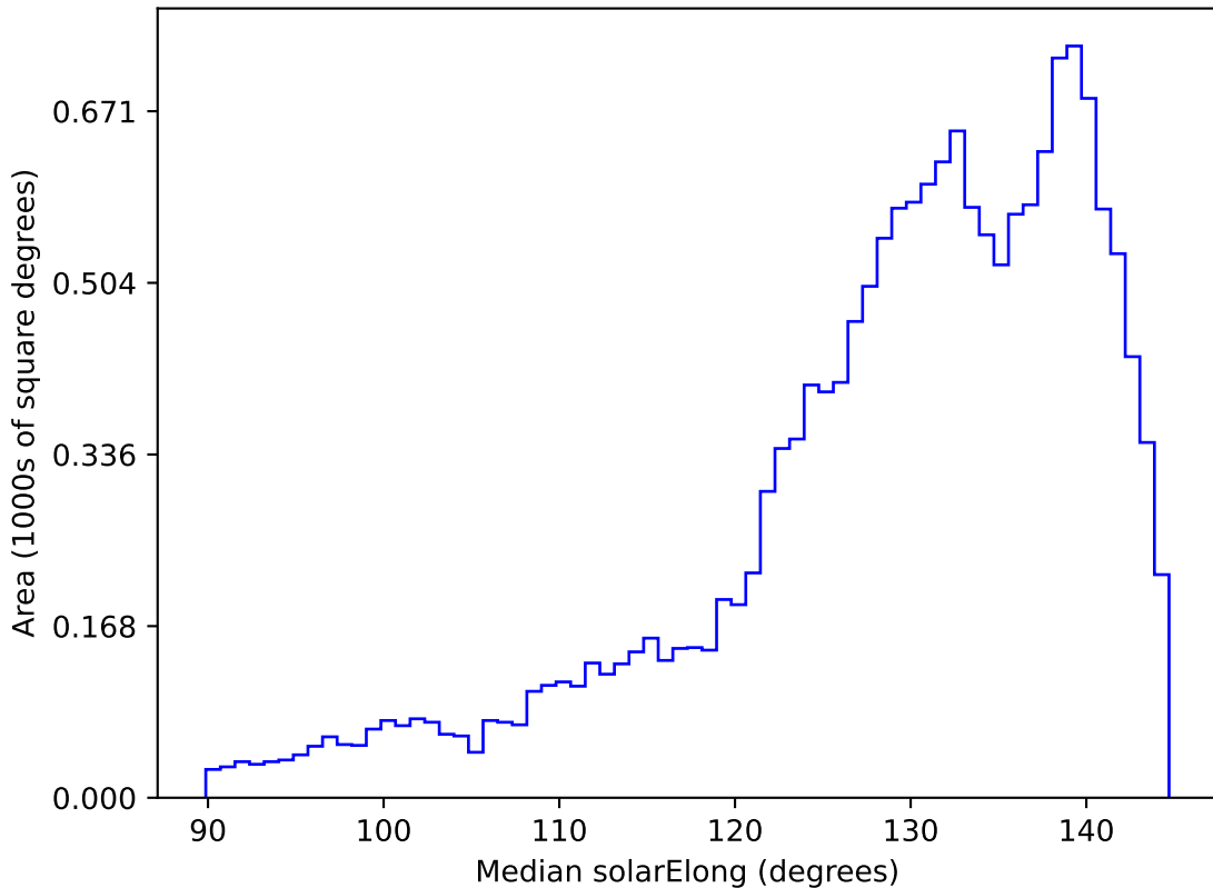
smc_lmc_v3.3_10yrs WFD all bands: Median solarElong
