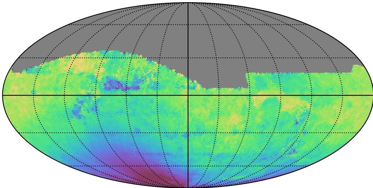
smc_lmc_v3.3_10yrs All sky z band: Median solarElong
