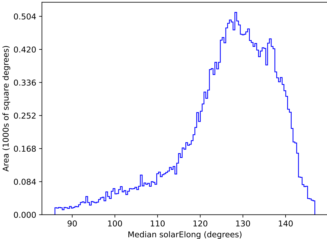
smc_lmc_v3.3_10yrs All sky z band: Median solarElong
