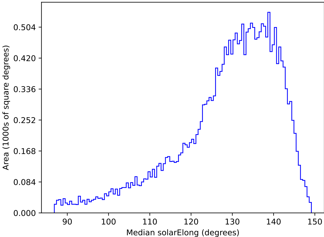
smc_lmc_v3.3_10yrs All sky y band: Median solarElong
