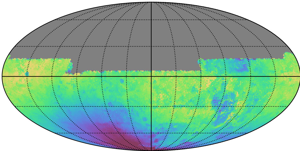
smc_lmc_v3.3_10yrs All sky u band: Median solarElong
