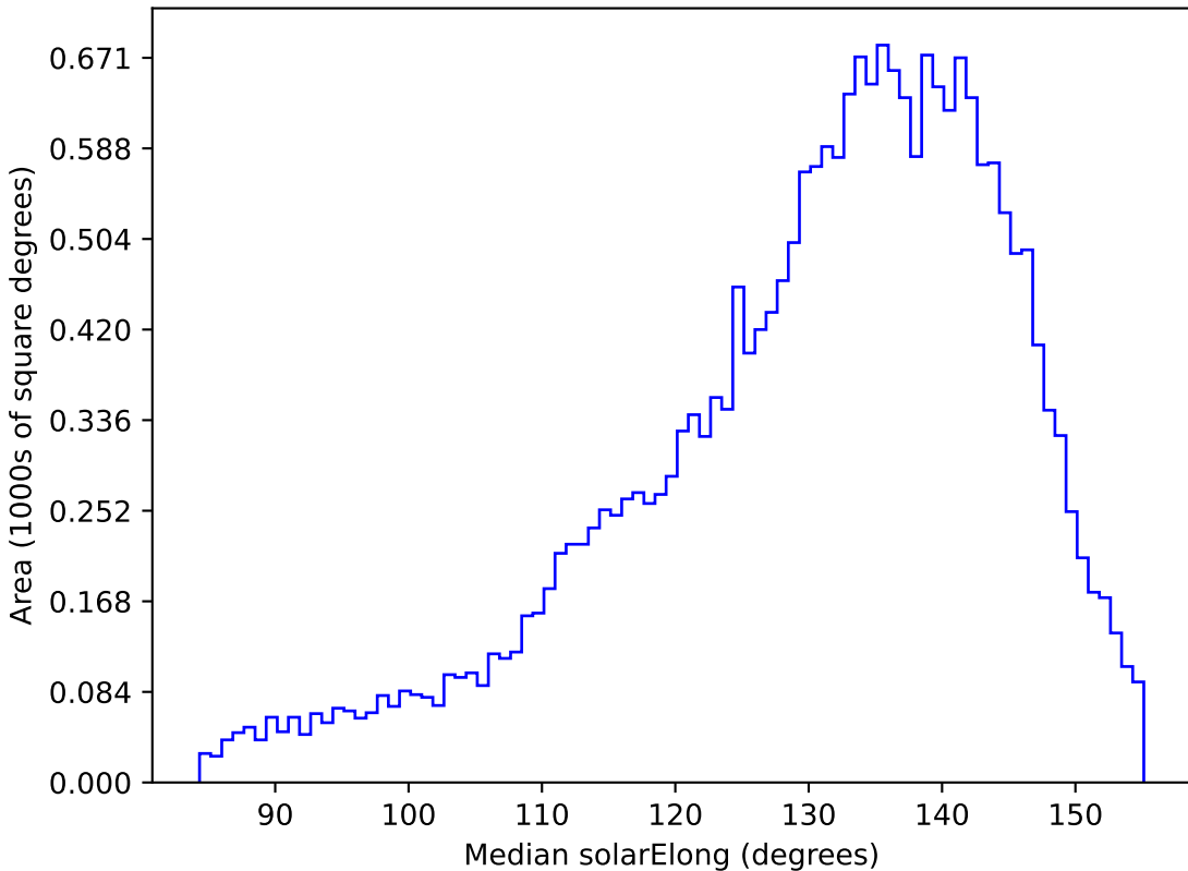
smc_lmc_v3.3_10yrs All sky u band: Median solarElong
