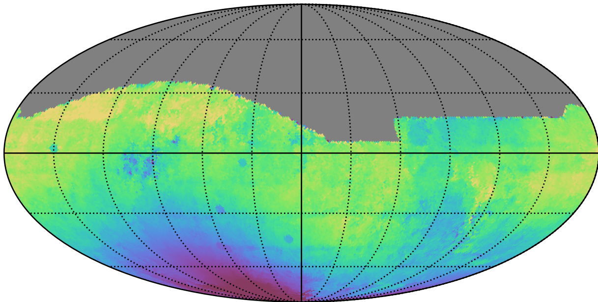
smc_lmc_v3.3_10yrs All sky r band: Median solarElong
