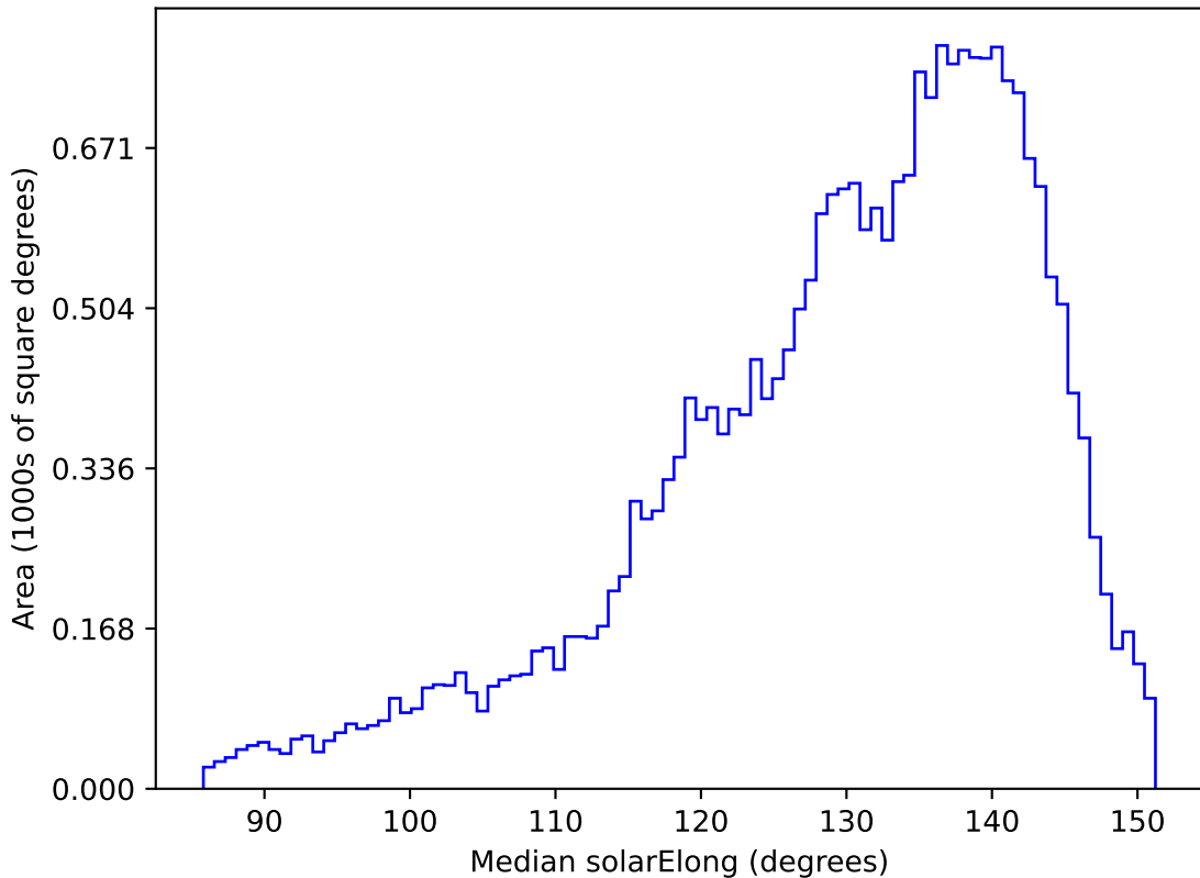
smc_lmc_v3.3_10yrs All sky r band: Median solarElong
