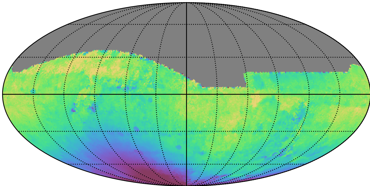
smc_lmc_v3.3_10yrs All sky i band: Median solarElong
