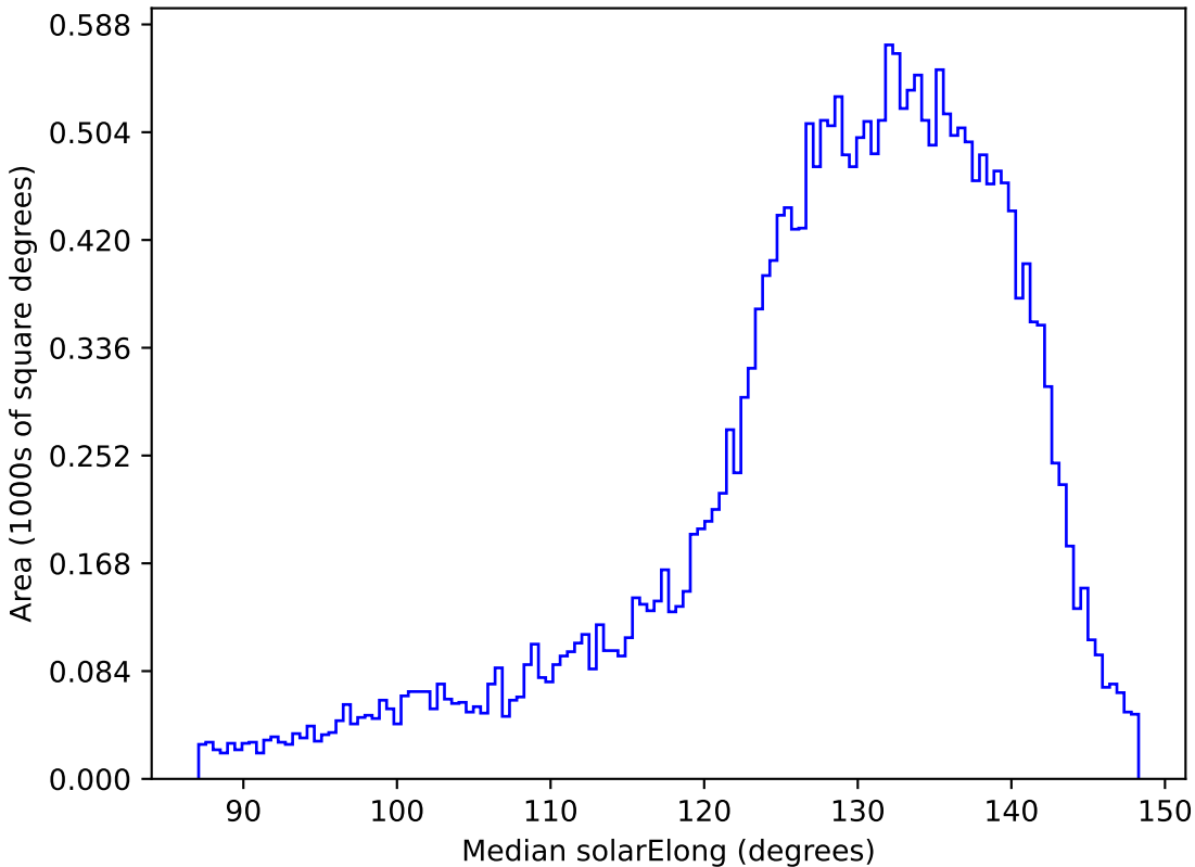
smc_lmc_v3.3_10yrs All sky i band: Median solarElong
