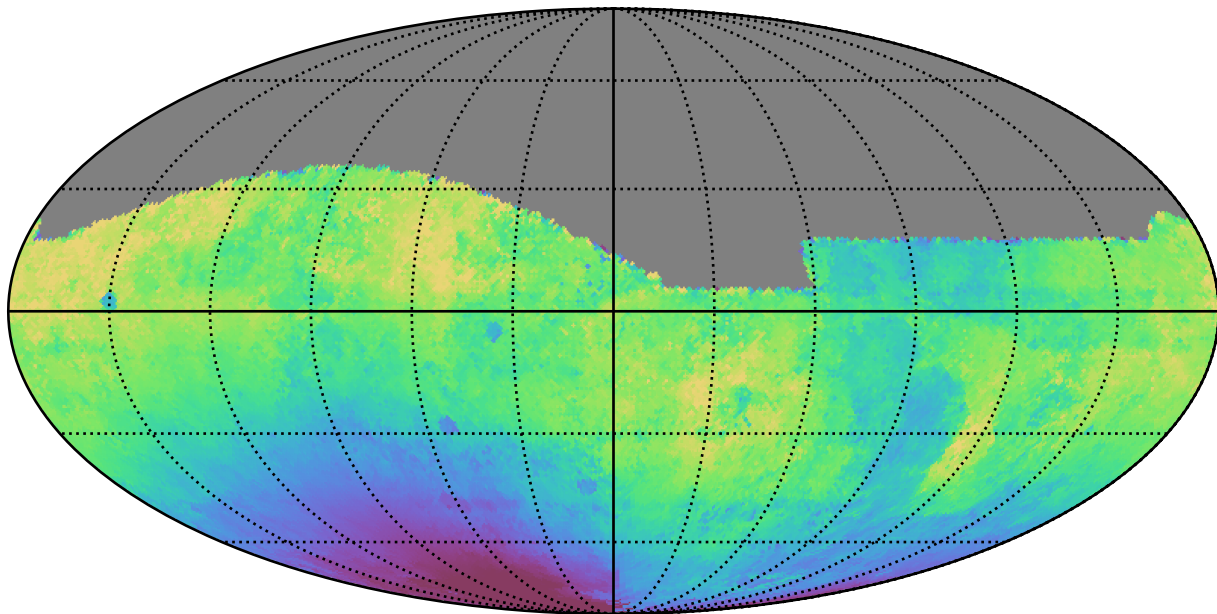
smc_lmc_v3.3_10yrs All sky g band: Median solarElong
