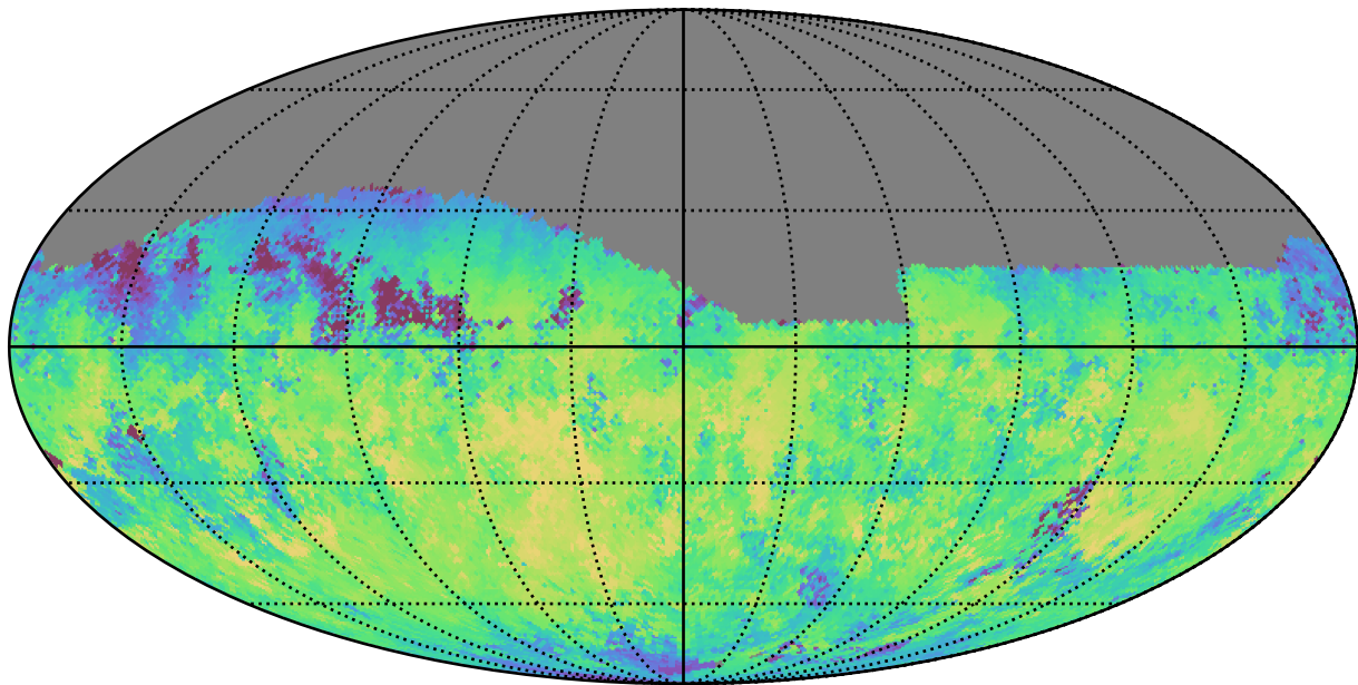
smc_lmc_v3.3_10yrs Yr 1 z band: Median skyBrightness
