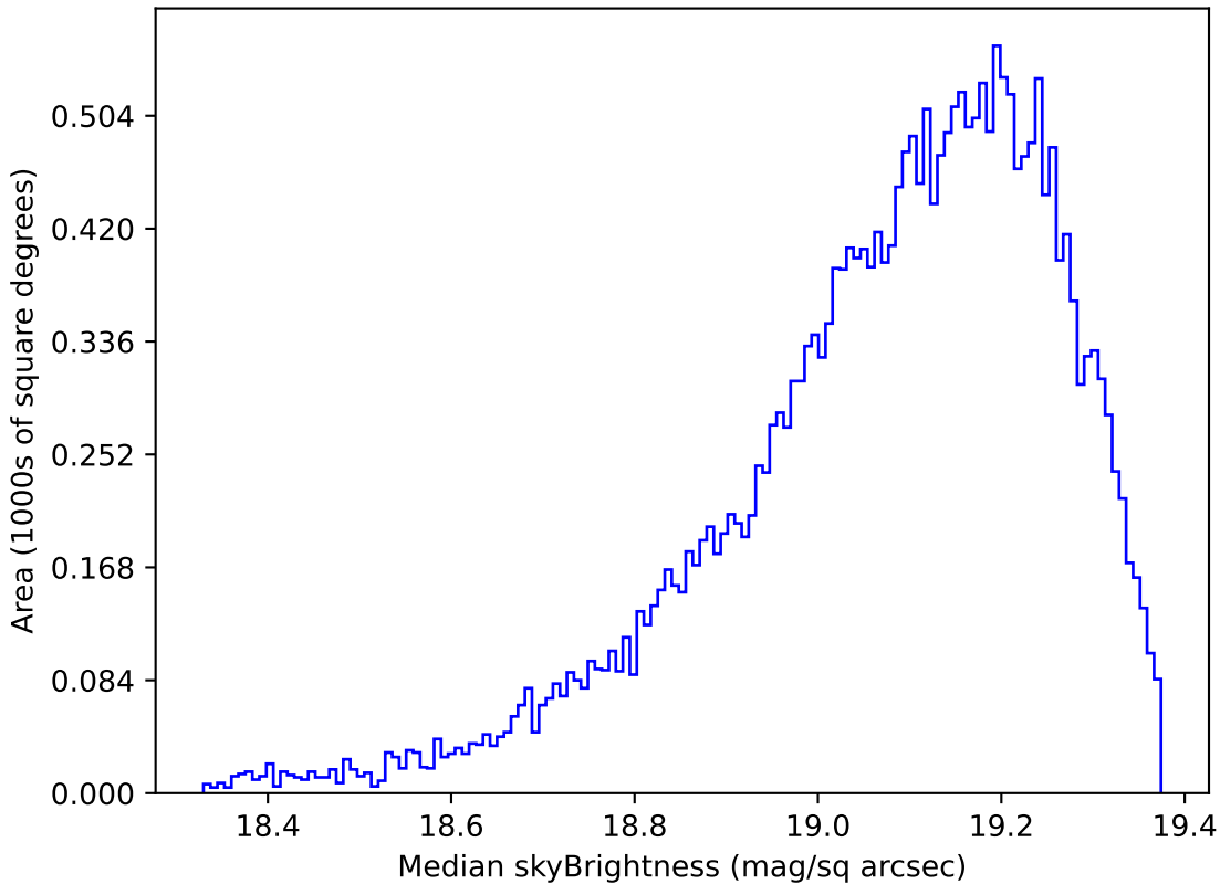
smc_lmc_v3.3_10yrs Yr 1 z band: Median skyBrightness
